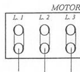
CONNECTION 220 V THREE-PHASE.
