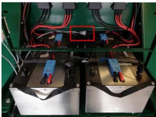
Figur 6: COM stik
