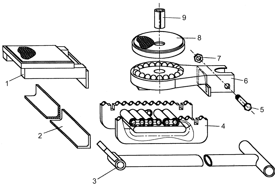
4.15 Exploded figure of SK20 and parts list
