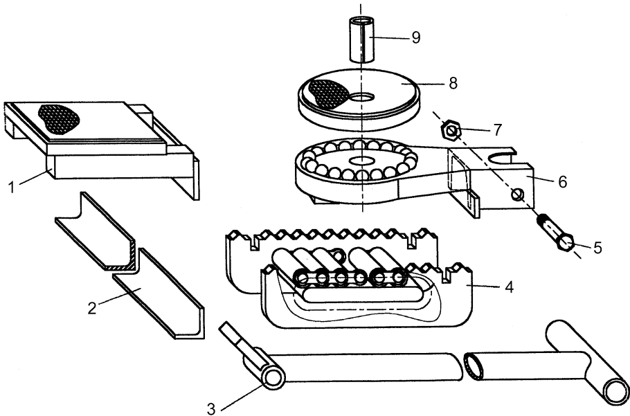
4.17 Exploded figure of SK60 and parts list
