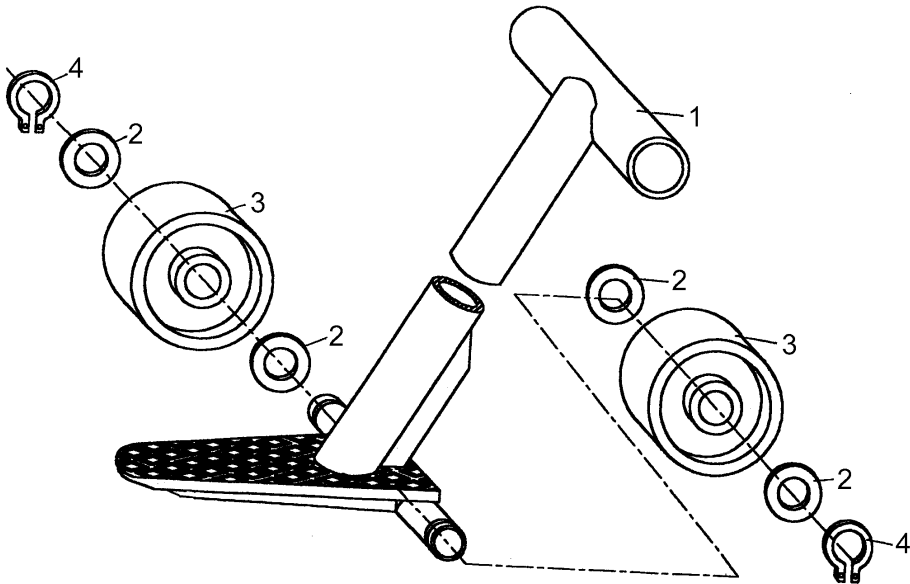
4.14 Exploded figure of RC15 and parts list
