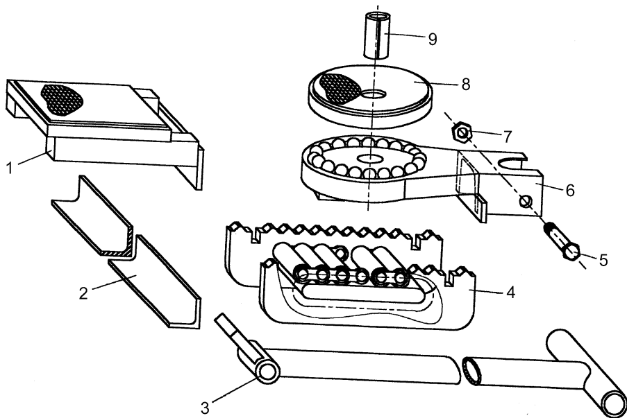
4.16 Exploded figure of SK30 and parts list
